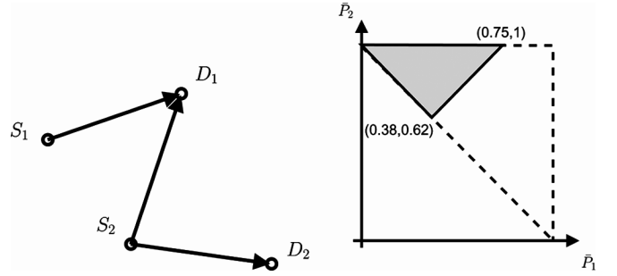
Fig. 6. Sensor example: On the left, an example of a network with two sensors and two sinks is given. We let P^M = N = 1 , and h_{S_1 D_1} = h_{S_1 D_2} = 1 , h_{S_2 D_1} = 10 , h_{S_2 D_2} = 0.7 , and the lower bounds on rates are M_1 = 0.6 , M_2 = 0.4 . On the right, the set of feasible average power dissipations is given.
