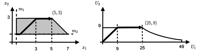
Fig. 2. More examples of feasible rate sets. We consider the topology given on the left of Fig. 1. We first assume there are minimum rates, m_1 = 0.5 and m_2 = 1 , for flows x_1 and x_2 , respectively. The feasible set for this case is depicted on the left. The water-filling [12], [27] is represented with the bold arrow. On the right we consider utility max-min fairness as defined in [8], [28] on the network from Fig. 1. The utility function is U(x) = x^2 . The set of feasible utilities (non-convex set) is depicted on the right and the water-filling is represented with the bold arrow.
