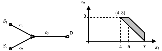
Fig. 4. When water-filling does not work—consider the network topology on the left ( c_1 = 7, c_2 = 3, c_3 = 8 ). Suppose that node D receives parts of the same stream from both S_1 and S_2 , through flows x_1 and x_2 , and suppose it needs a minimal total rate of x_1 + x_2 \geq 7 . We want to minimize loads of servers S_1 and S_2 , and we are interested in min-max fair allocation of (x_1, x_2) . The feasible rates set is given on the right. Min-max fair allocation exists, and it is (4, 3) .
