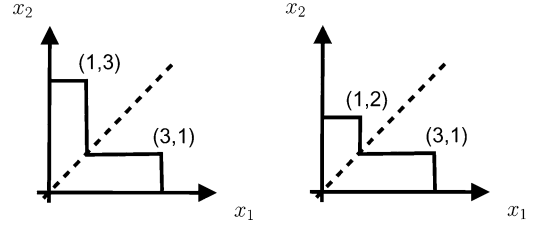
Fig. 5. Examples of two-dimensional sets that do not have max-min fair allocation. Point (1, 3) is not max-min fair in the example on the left since there exists point (3, 1) that contradicts Definition 1. Both points (1, 3) and (3, 1) are leximin maximal in this example. In the example on the right, point (3, 1) is the single leximin maximal point. Still, it is not the max-min fair point. Note that there exists no real networking example we are aware of that has these feasible rate sets—these sets are only artificial examples that illustrate properties of leximin ordering.
