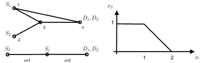
Fig. 3. Simple multi-path example. Top-left: S_1 sends to D_1 over two paths, 1-3-4 and 1-4, while S_2 sends to D_2 over a single path 2-3-4. All links have capacity 1. Right: the set of feasible rates. Bottom-left: the corresponding virtual single path problem.
