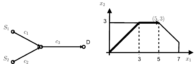
Fig. 1. Example of a feasible rate set and water-filling. On the left, a network of three links is given. Flow x_1 connects S_1 and D and flow x_2 connects S_2 and D . The set of feasible rates (x_1, x_2) is given on the right ( c_1 = 7, c_2 = 3, c_3 = 8 ). The water-filling [7] is depicted by the bold arrow. The max-min fair rate allocation is (5, 3) .
